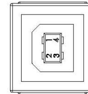
P2 USB TYPE B FEMALE JACK
